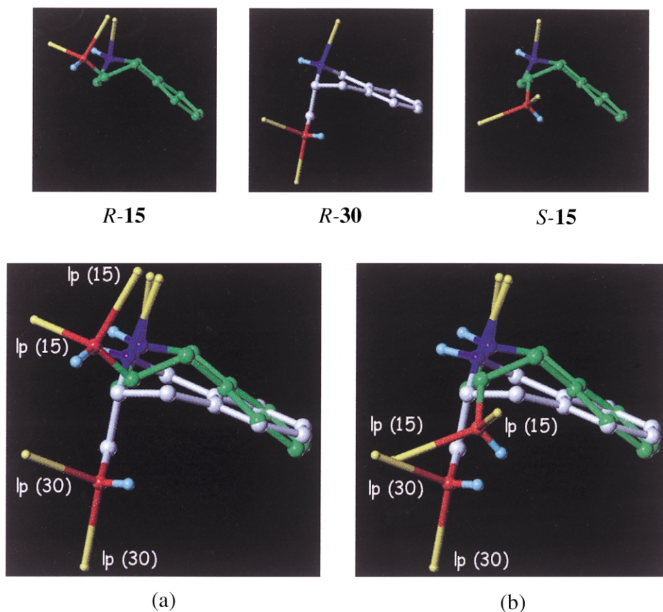
Figure 1. Superimpositions of the enantiomers of 15 (green; a: R and b: S ) over the more active (at PNMT) enantiomer of 30 (white; R ). Compounds were superimposed using both ends of a 2 Å long normal through the centroid of the aromatic ring and the end of the axial lone pair (2.4 Å) from the THIQ or THBA nitrogen. Hydroxyl oxygens are shown in red, hydroxyl hydrogens are in cyan, and lone pairs are in yellow. The hydrogens on the carbon skeleton have been deleted for clarity.
