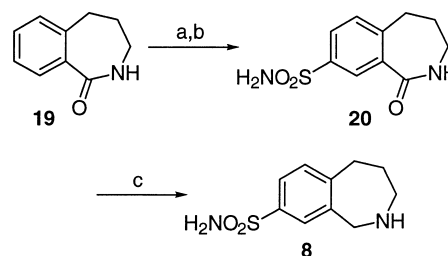
Scheme 2. Reagents and conditions: (a) ClSO 3 H; (b) NH 4 OH; (c) BH 3 THF, reflux.
